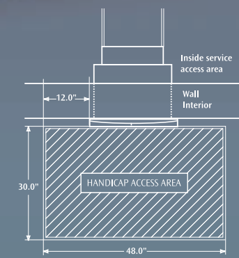
ATM INSTALLATION SPACE REQUIREMENTS FOR ADA COMPLIANCE
